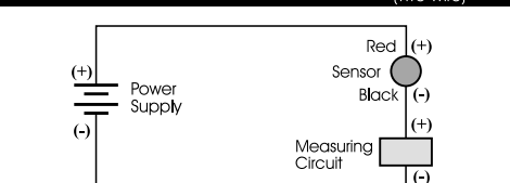
Current Output Sensor Wiring Configuration
