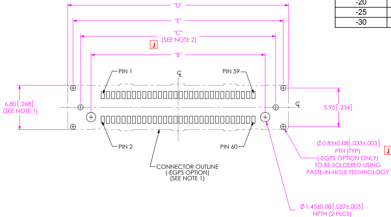
FIG 3 -EGPS OPTION (-030 POSITION SHOWN) (SAME AS FIG 1, EXCEPT AS SHOWN) (ALL DIMENSIONS ARE SYMMETRIC ABOUT THE CENTERLINE)
